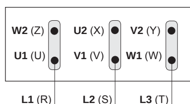
Δ Connection
